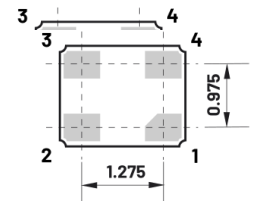
pads viewed from bottom pad size (0.72 x 0.55)mm
